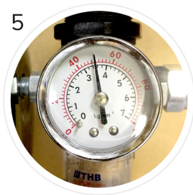
After inserting the grip, please raise the air pressure to 0.25 kg / cm 2.
